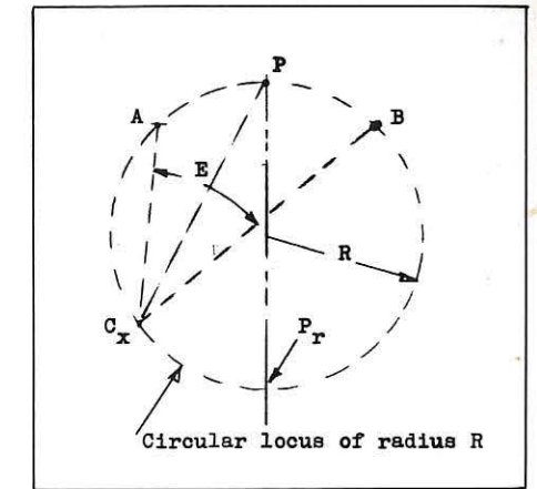
Figure 3: Plan view of capture system with arbitrary camera C_x .
